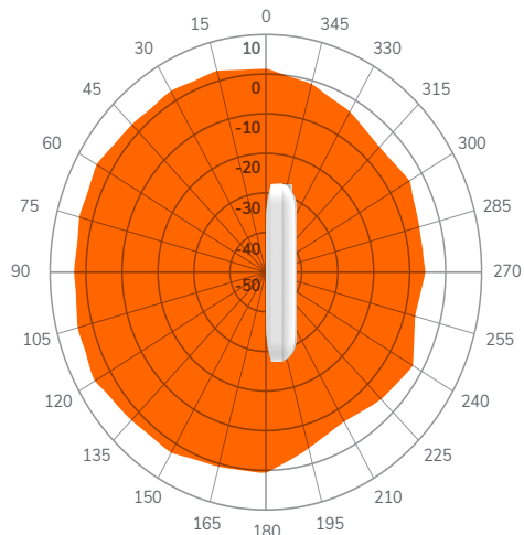
5 GHz, XY-Ebene
