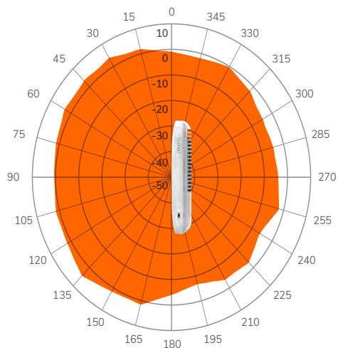
5 GHz, YZ-Ebene
