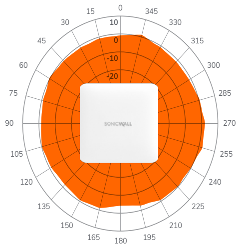
5 GHz, XY-Ebene
