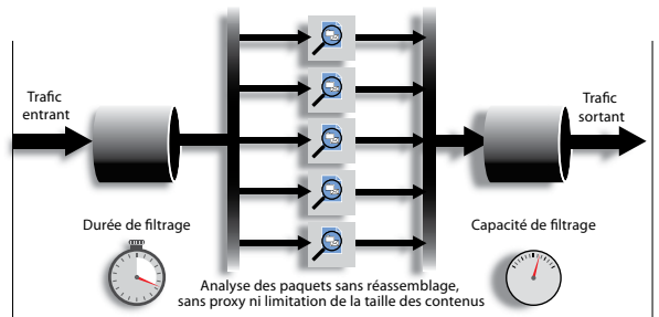
Architecture SonicWALL
